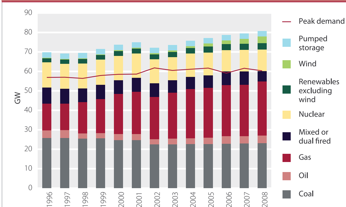
Figure 4.3 Installed capacity (1996-2008)
