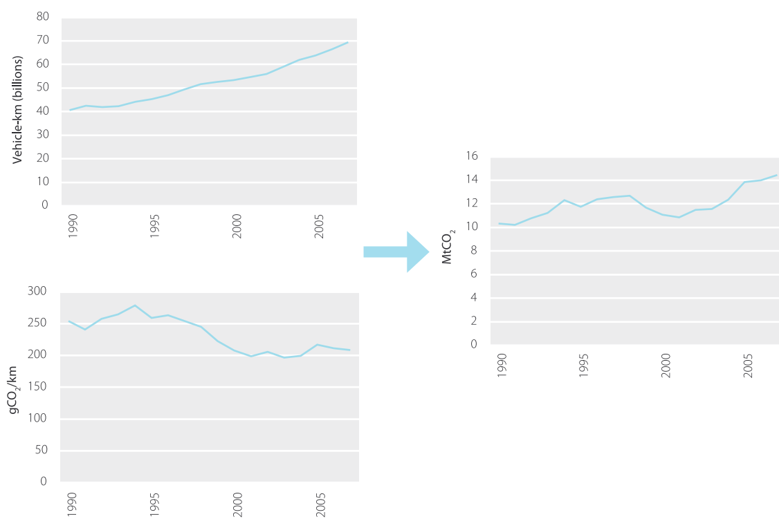
Figure 6.5 Historical trends in vehicle km, CO 2 and gCO 2 /km for vans 1990 – 2007
