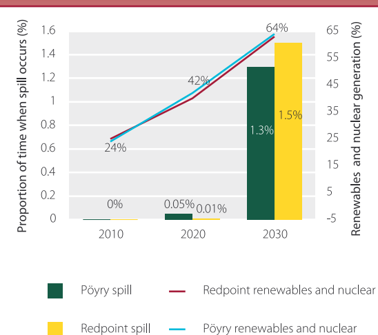
Figure 4.7 Spill with high levels of wind and nuclear
