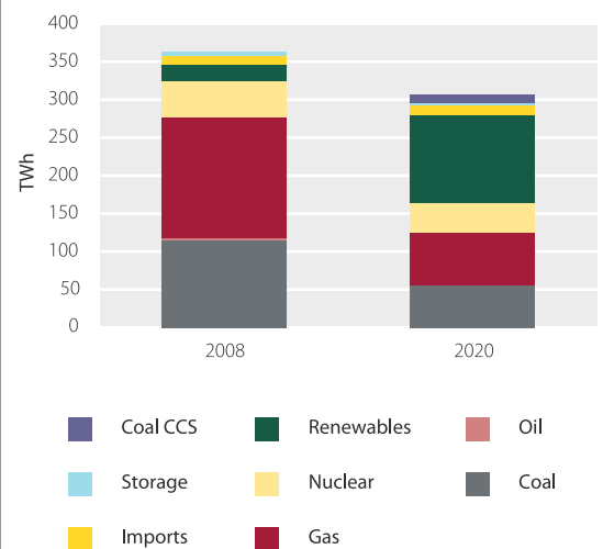
Figure 4.9 CCC scenario for generation mix in 2020 compared to actual generation mix in 2008
