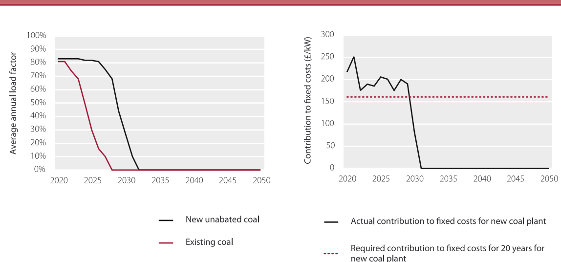
Figure 4.22 Projected load factors and profitability for conventional coal
