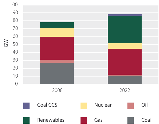
Figure 4.8 CCC scenario for capacity mix in 2020 compared to actual capacity mix in 2008
