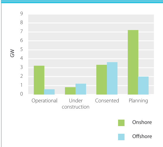
Figure 2.12 Wind projects according to various stages of development, September 2009
