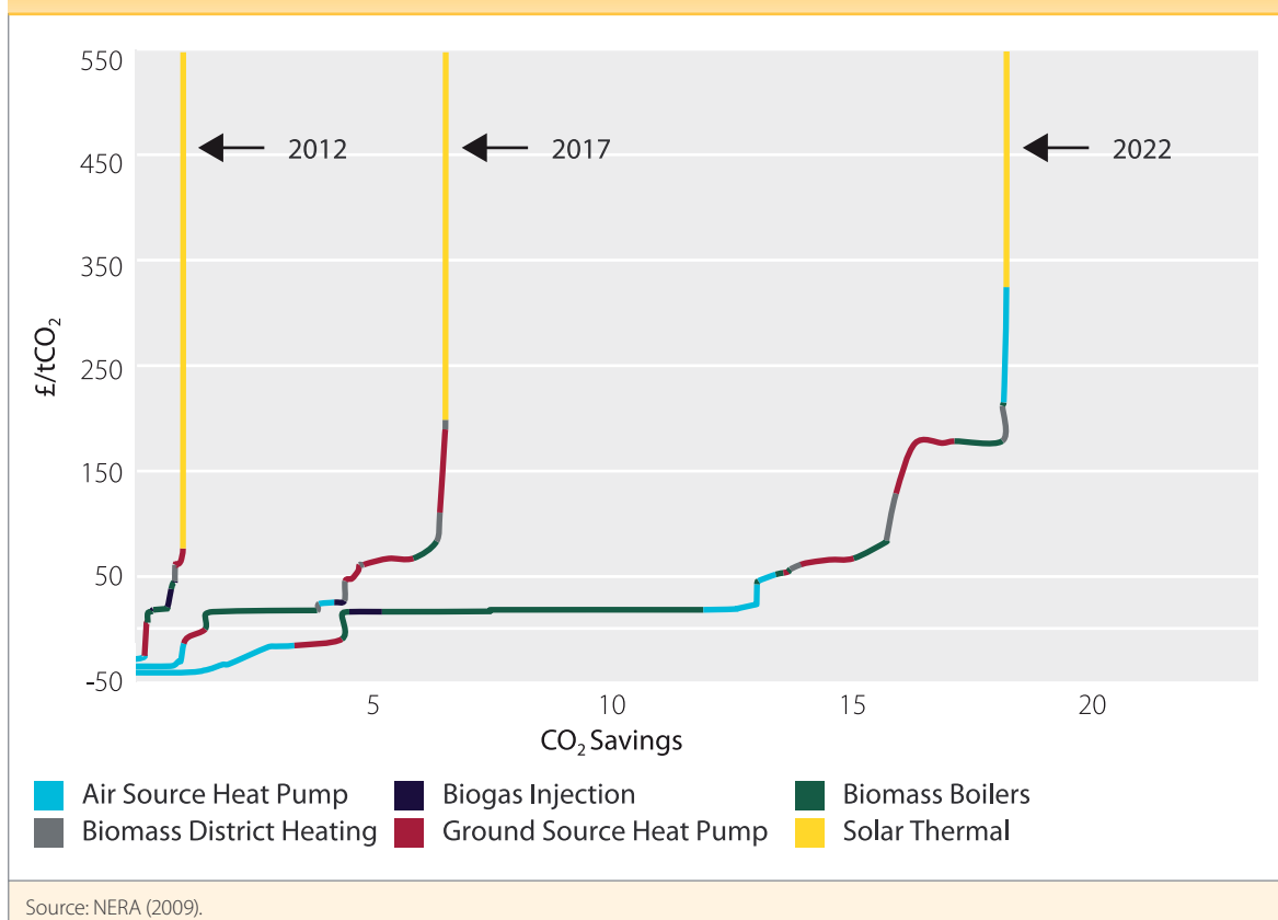
Figure 5.18 MACC showing penetration in the central scenario over time
