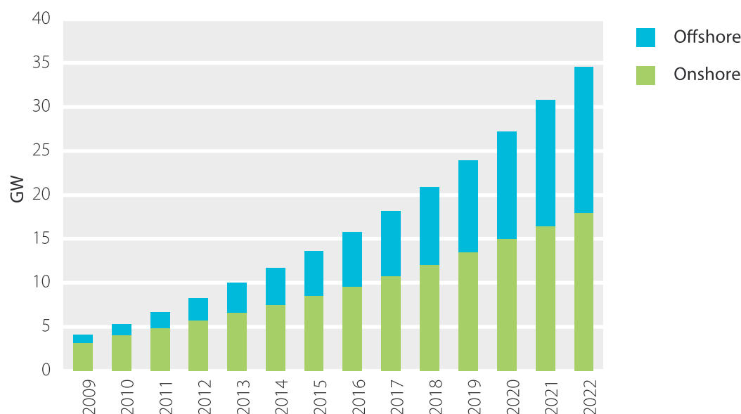
Figure 4.13 Operational wind capacity in the high feasible scenario
