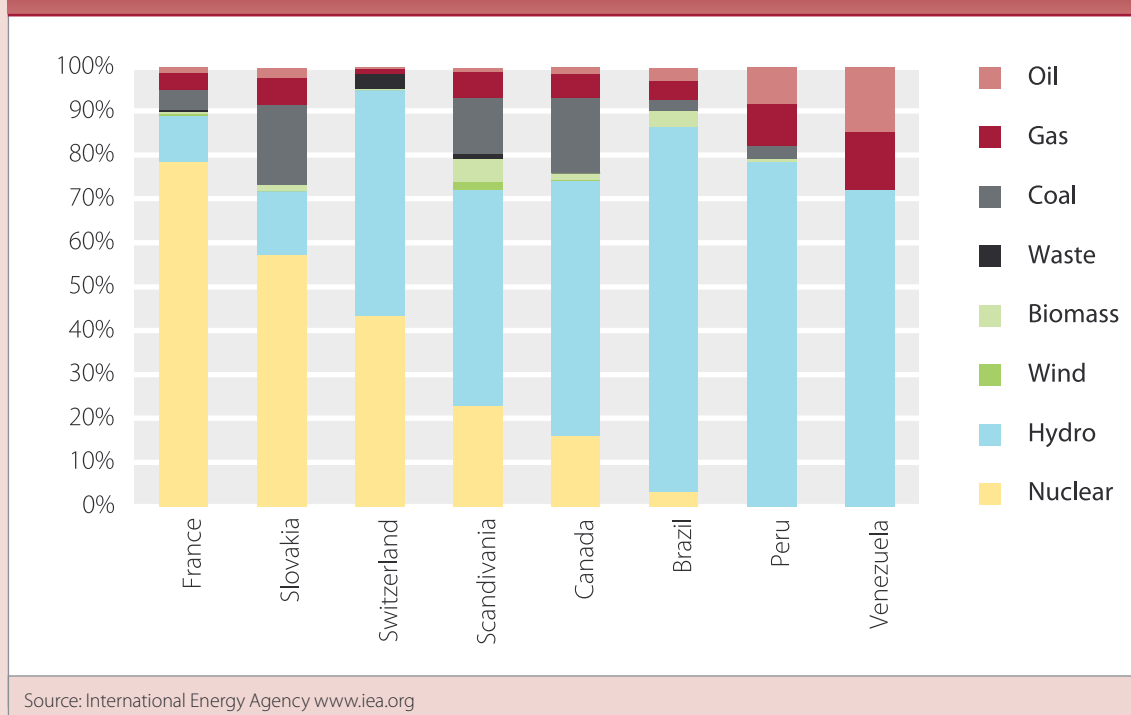
Figure B4.10 Generation mix in predominantly low-carbon electricity markets (2006)
