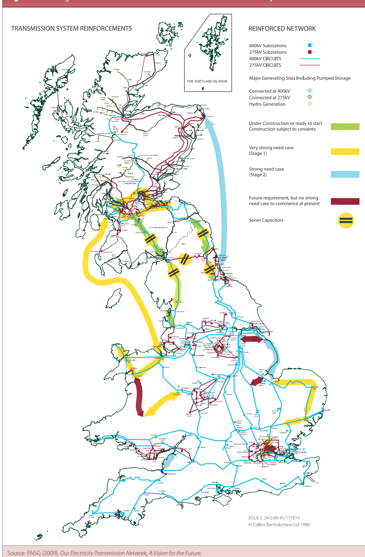
Figure 4.15 Stage 1 and 2 transmission reinforcements recommended by ENSG
