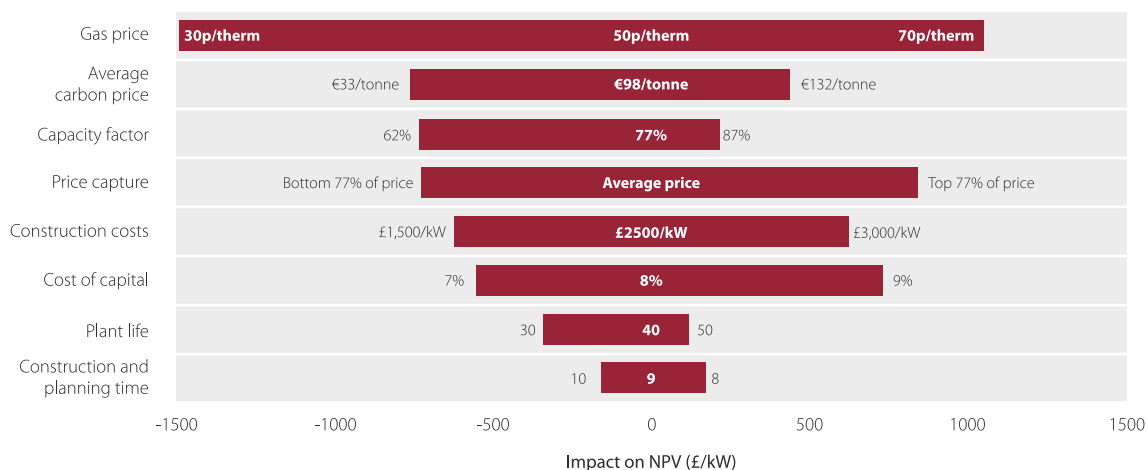
Figure 4.26 Relative importance of uncertainties faced by nuclear investors
