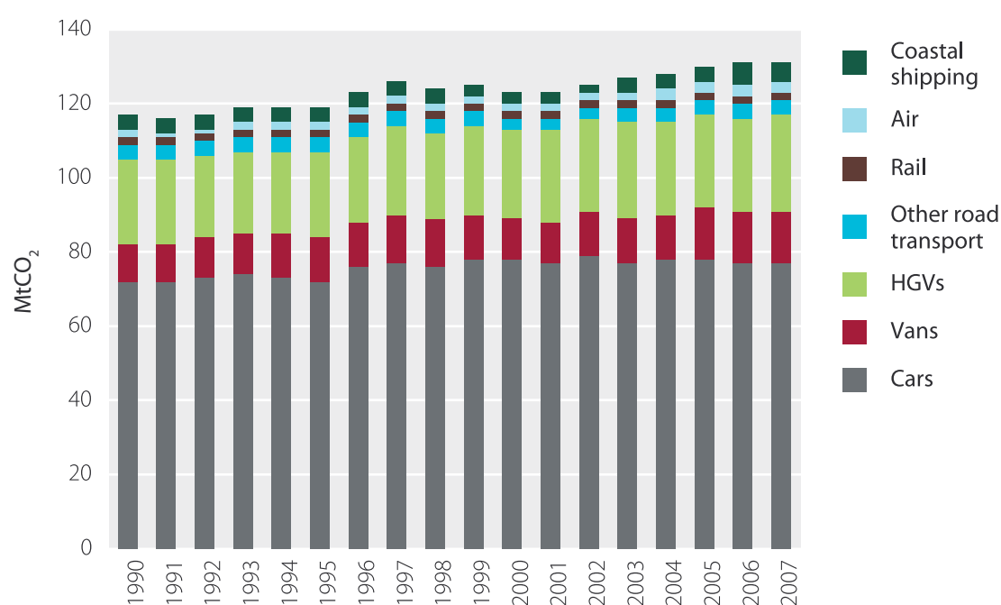
Figure 1.13 CO 2 emissions from transport by mode 1990-2007
