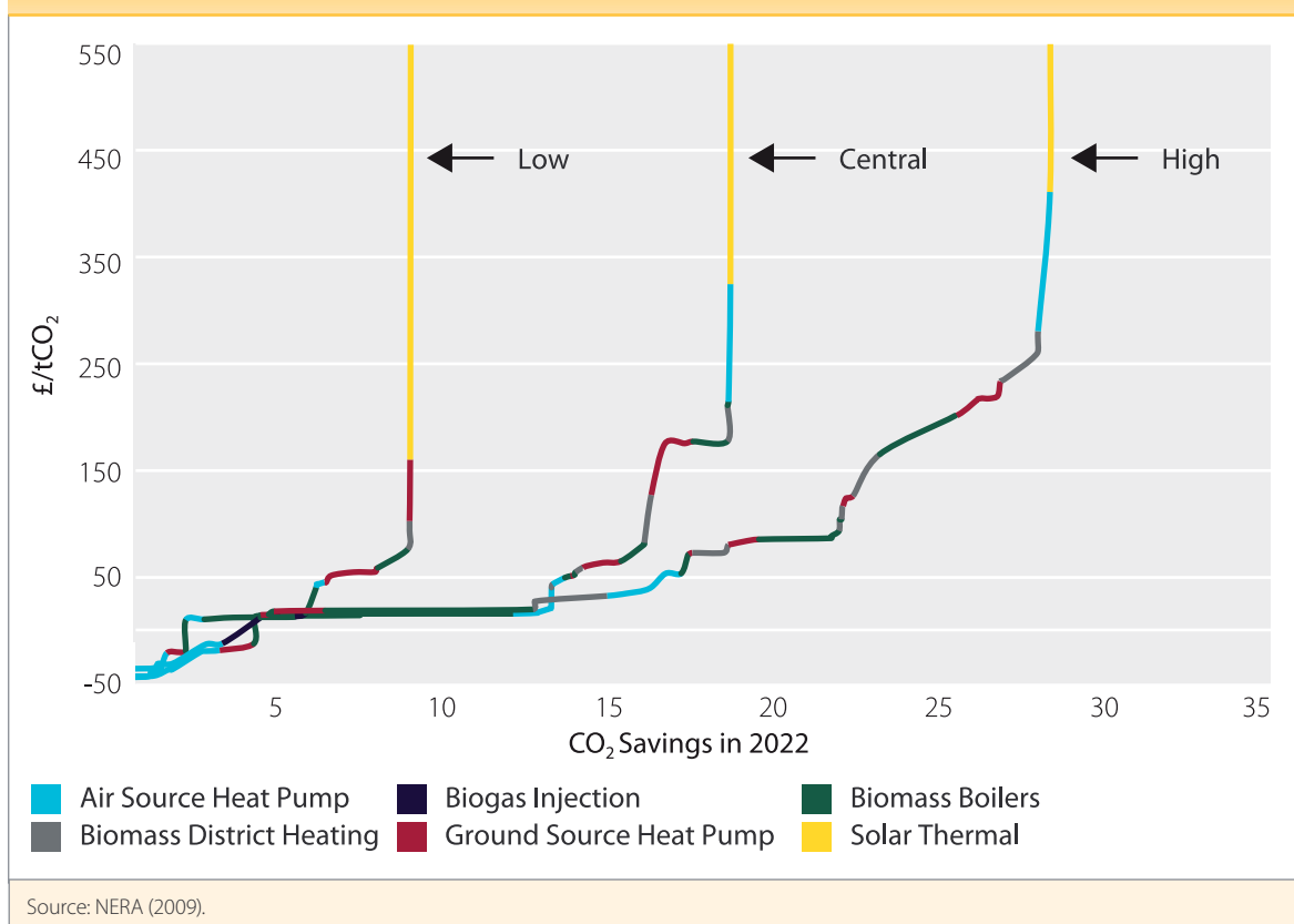
Figure 5.17 MACC for low, central and high scenarios in 2022
