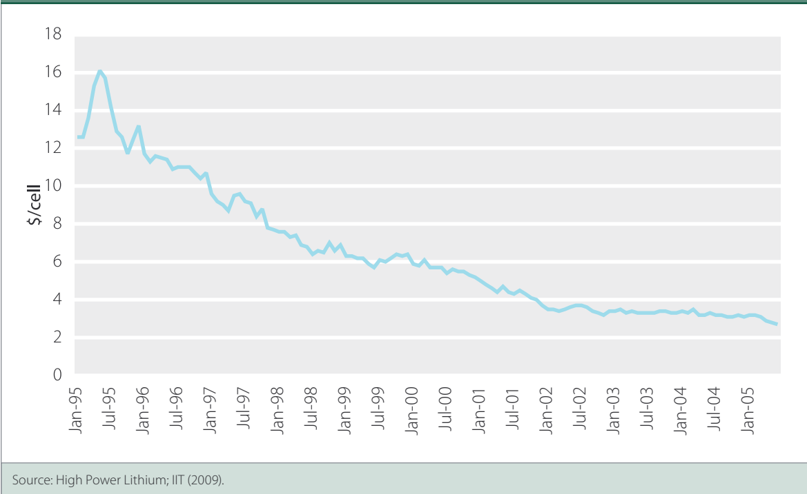
Figure 6.17 Cost of Japanese manufactured lithium-ion laptop battery cells 1995-2005
