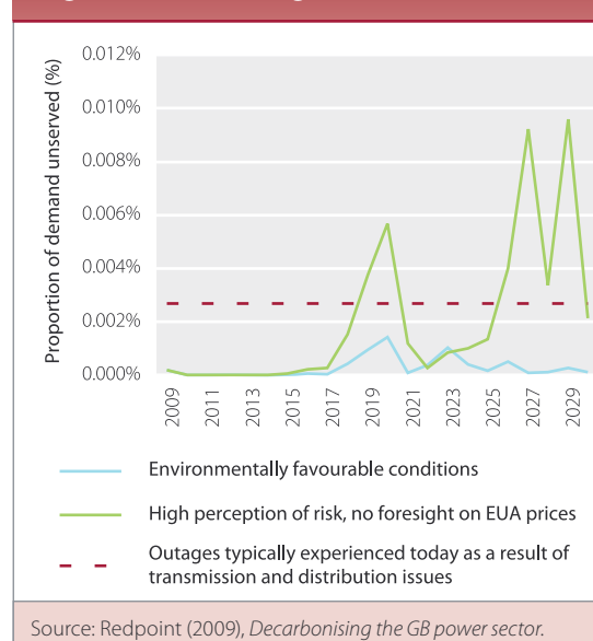
Figure 4.27 Expected energy unserved due to generation shortage
