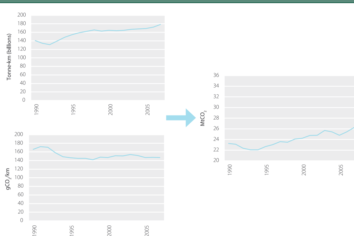
Figure 6.7 Historical trends in tonne-km, CO 2 and gCO 2 /tonne-km for HGVs 1990 – 2007
